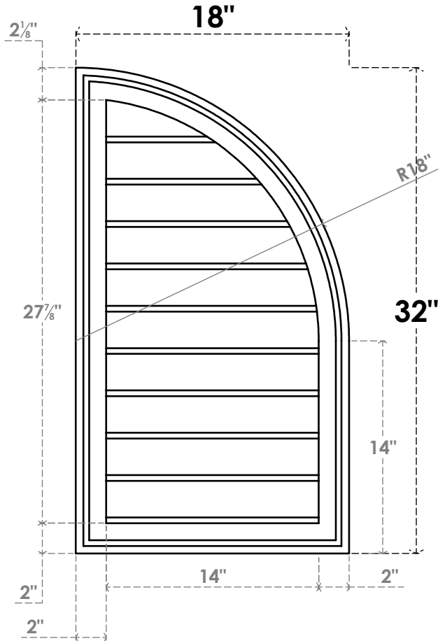
FRONT
